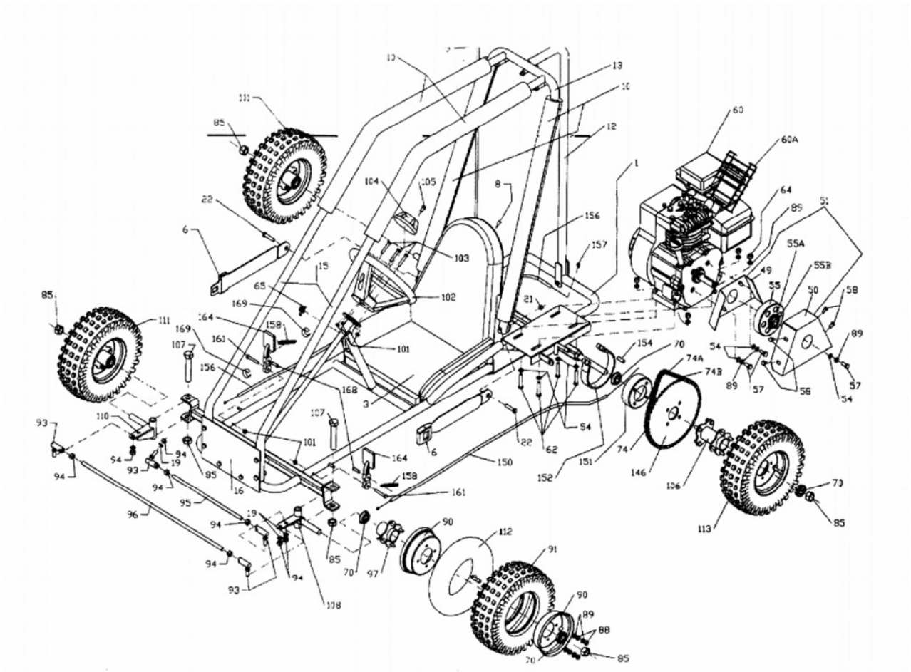
Figure 1 Schematic diagram of Kartco models 300 and 335
